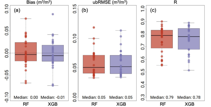
Fig. 6. Boxplots of (a) bias, (b) ubRMSE, and (c) R for a fourfold spatial CV of RF and XGB models, respectively, between January 1, 2016 and December 31, 2019. The details of sites included in each fold are given in Table II. The scatters represent the metrics of individual sites.
